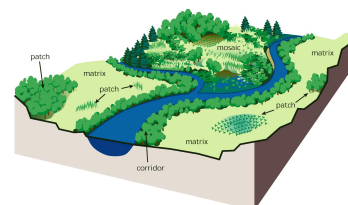
Fig. 1.4 - Spatial structure. Landscapes can be described in terms of matrix, patch, corridors and corridor-in-matrix patches. From: Forman, 1995.
